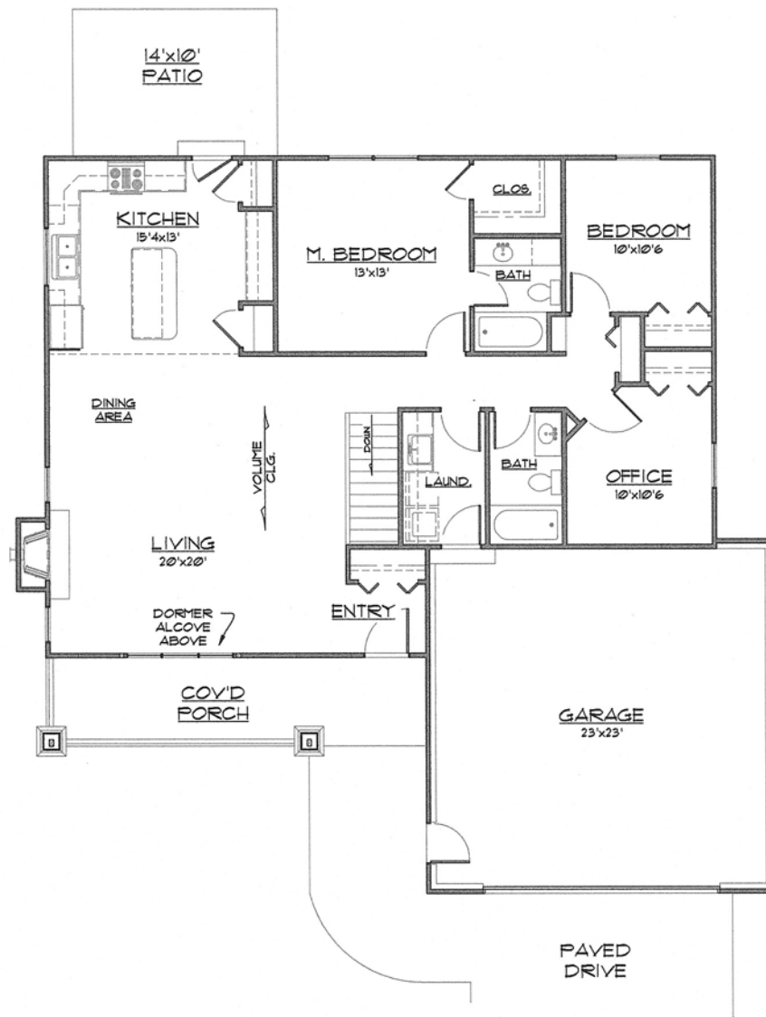
FLOOR PLAN
