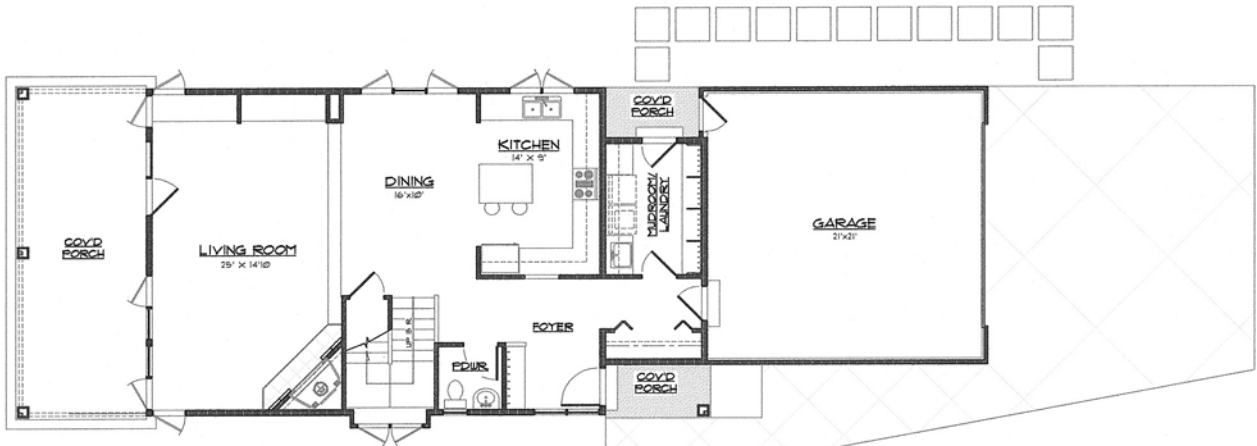
MAIN LEVEL PLAN
